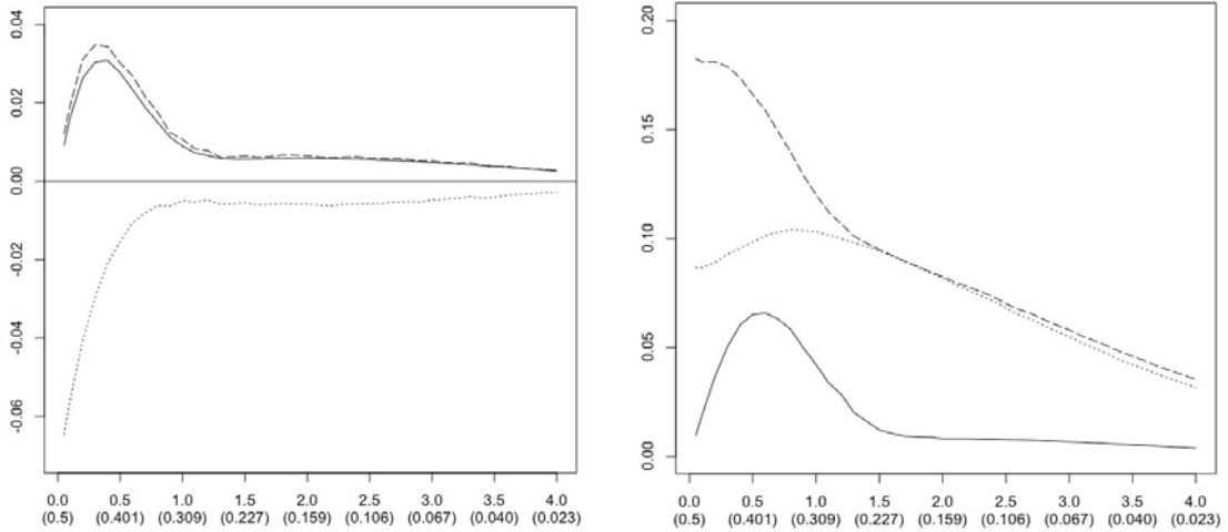
Figure 9. Error estimator performance for LDA in one-dimensional Gaussian model based on Glick’s paper; (a) (1) E[\varepsilon_{LDA}(m)] - \varepsilon_{bay}(m) (solid), (2) E[\hat{\varepsilon}^{res}(m)] - \varepsilon_{bay}(m) (dots), and (3) E[\hat{\varepsilon}^{loo}(m)] - \varepsilon_{bay}(m) (dashes); (b) \varepsilon_{LDA}(m) (solid), \hat{\varepsilon}^{res}(m) (dots), and \hat{\varepsilon}^{loo}(m) (dashes).
