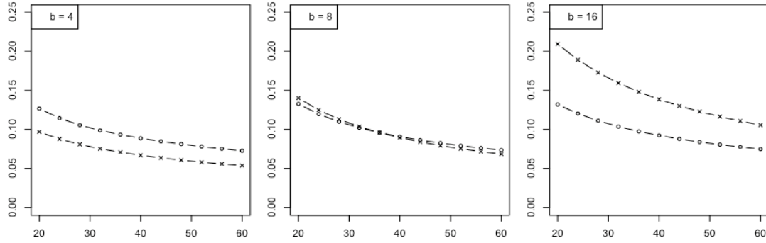
Figure 10. RMS versus sample size for discrete classification: (x) resubstitution; (o) leave-one-out.
