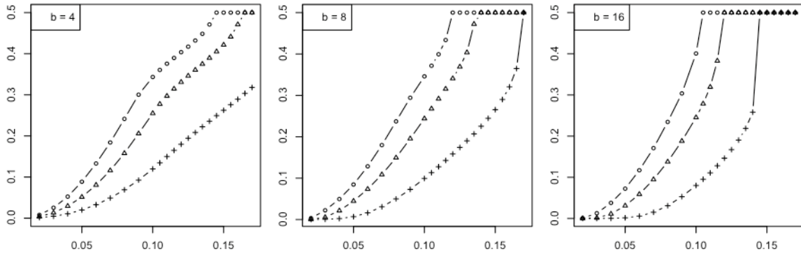
Figure 8. Maximum Bayes error versus \text{RMS} = \lambda for leave-one-out for discrete classification: (+) is n = 20 ; ( \Delta ) is n = 40 ; (o) is n = 60 .
