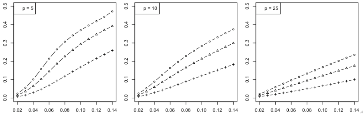
Figure 3. Maximum Bayes error versus \text{RMS} = \lambda for resubstitution in a Gaussian model: (+) is n = 20 ; ( \Delta ) is n = 40 ; (o) is n = 60 .
