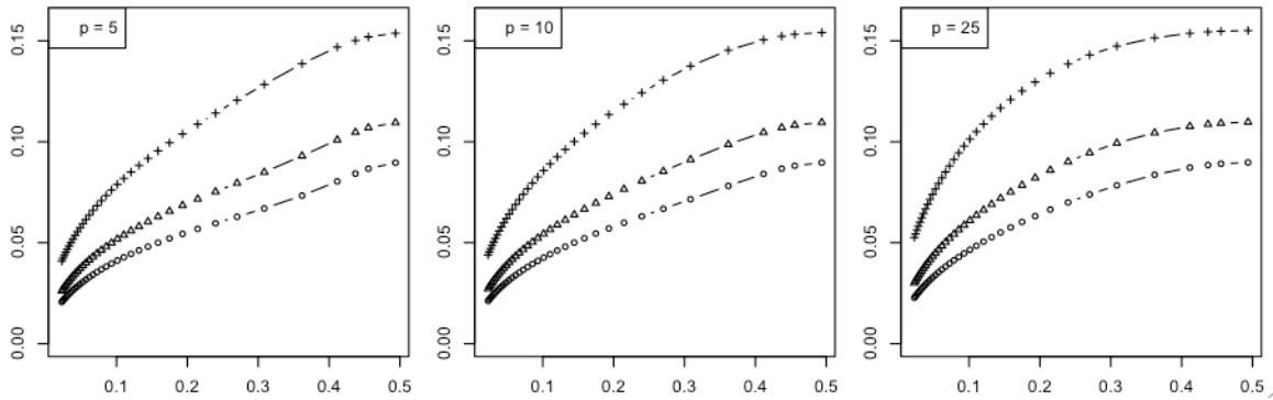
Figure 2. RMS versus Bayes error for leave-one-out in a Gaussian model: (+) is n = 20 ; ( \Delta ) is n = 40 ; (o) is n = 60 .
