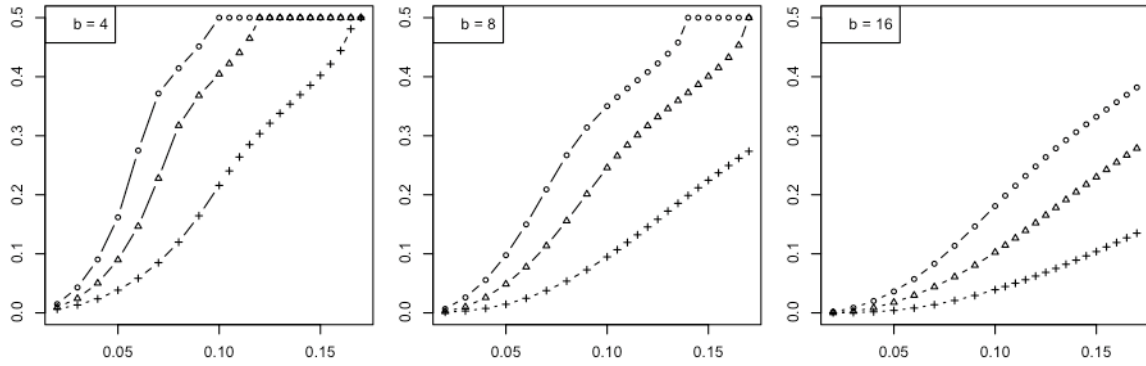
Figure 7. Maximum Bayes error versus \text{RMS} = \lambda for resubstitution for discrete classification: (+) is n = 20 ; ( \Delta ) is n = 40 ; (o) is n = 60 .
