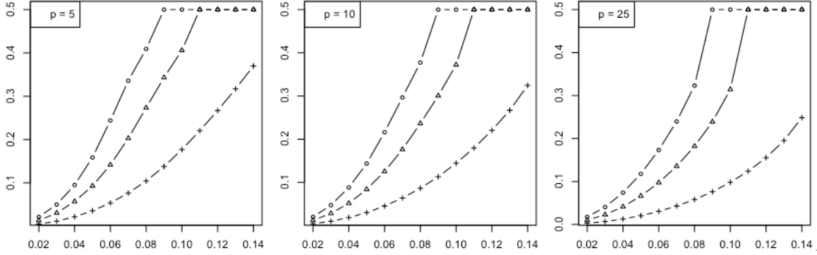
Figure 4. Maximum Bayes error versus \text{RMS} = \lambda for leave-one-out in a Gaussian model: (+) is n = 20 ; ( \Delta ) is n = 40 ; (o) is n = 60 .
