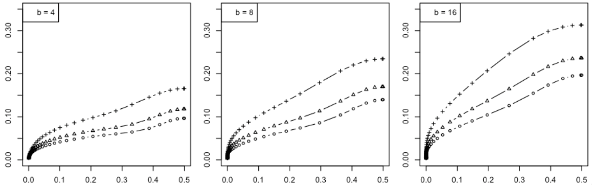
Figure 5. RMS versus Bayes error for resubstitution for discrete classification: (+) is n = 20 ; ( \Delta ) is n = 40 ; (o) is n = 60 .
