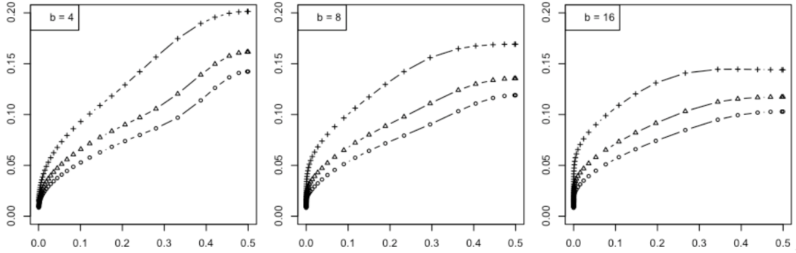
Figure 6. RMS versus Bayes error for leave-one-out for discrete classification: (+) is n = 20 ; ( \Delta ) is n = 40 ; (o) is n = 60 .
