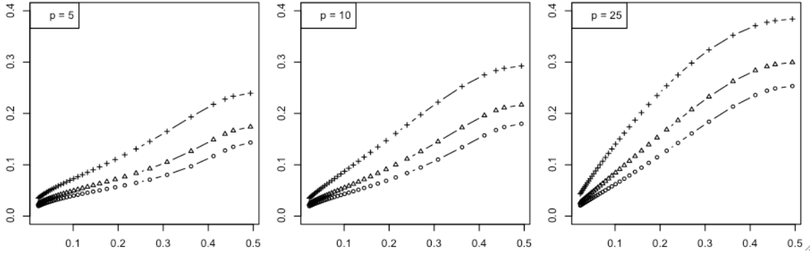
Figure 1. RMS versus Bayes error for resubstitution in a Gaussian model: (+) is n = 20 ; ( \Delta ) is n = 40 ; (o) is n = 60 .
